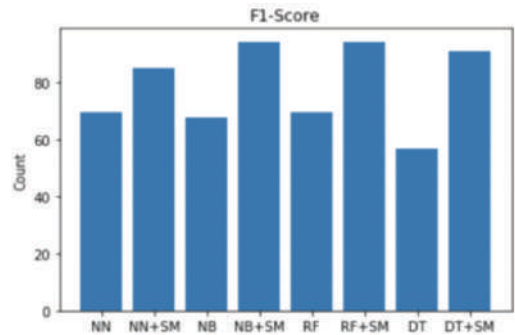
FIGURE 12 | F1-score result.
