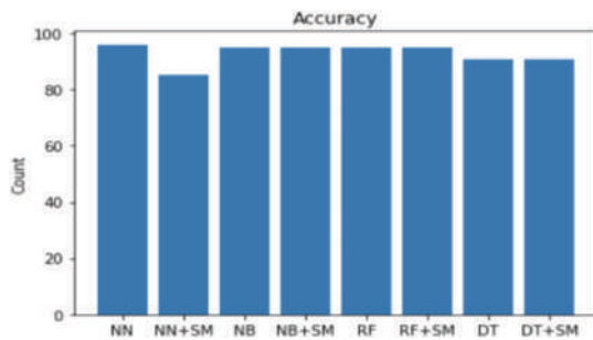
FIGURE 9 | Accuracy result.
