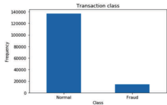
FIGURE 7 | Ratio fraud.
