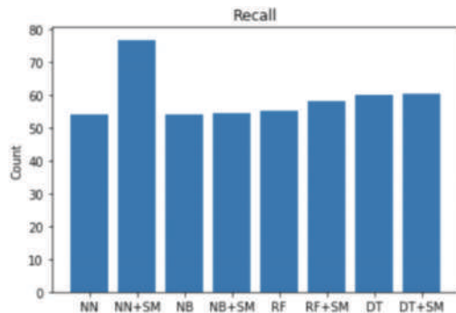
FIGURE 10 | Recall result.
