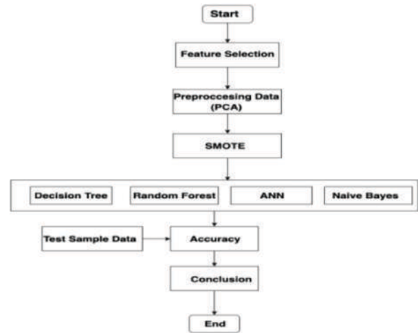
FIGURE 3 | Research steps.
