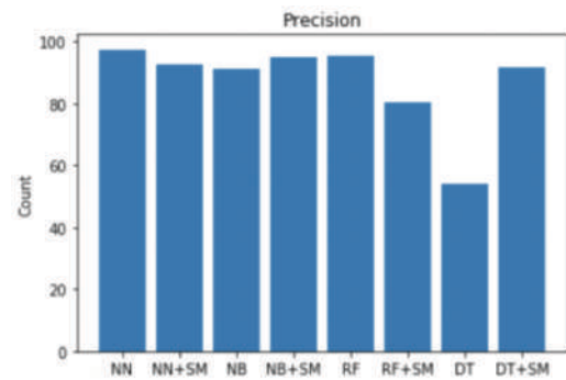
FIGURE 11 | Precision result.
