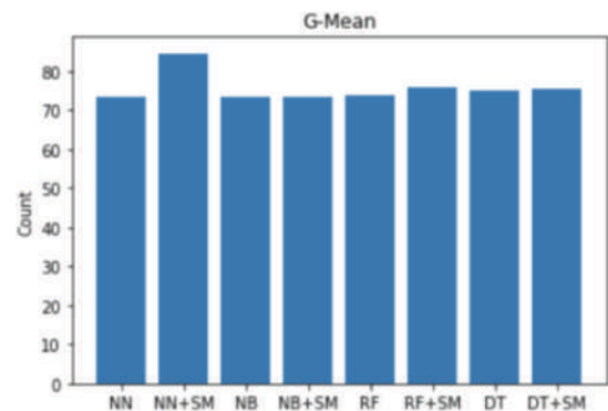
FIGURE 13 | G-mean result.
